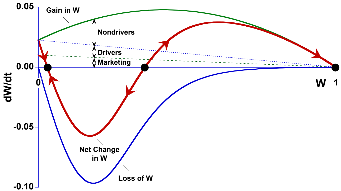
Figure 4 Phase plot for one-dimensional system showing two stable and one unstable fixed points for willingness to consider ICE drivers with AFVs (parameters in Table 2).
