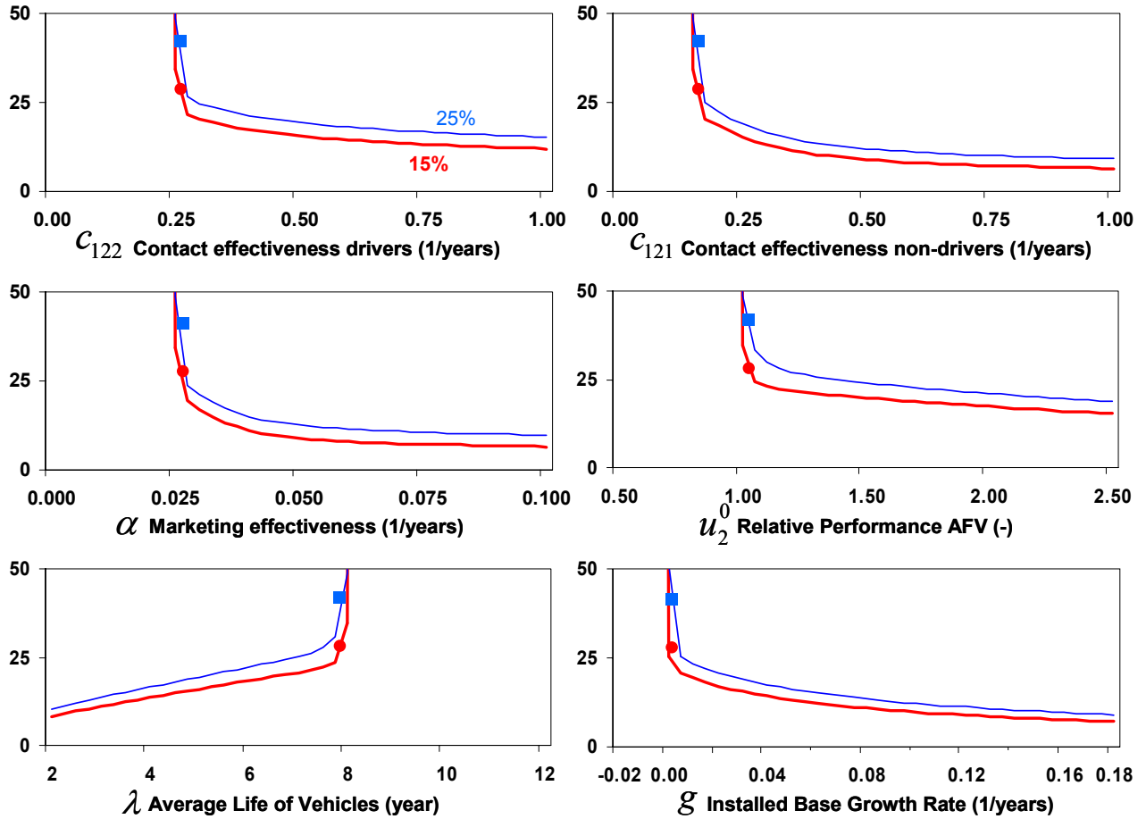
Figure 7 Sensitivity of the AFV installed base share to key parameters. Each panel shows the time required to achieve 15% and 25% share of the total installed base. The reference points (dots for 15% and squares for 25% market share) indicate the values for base run Figure 6 with an aggressive promotion and subsidy program lasting 20 years.
