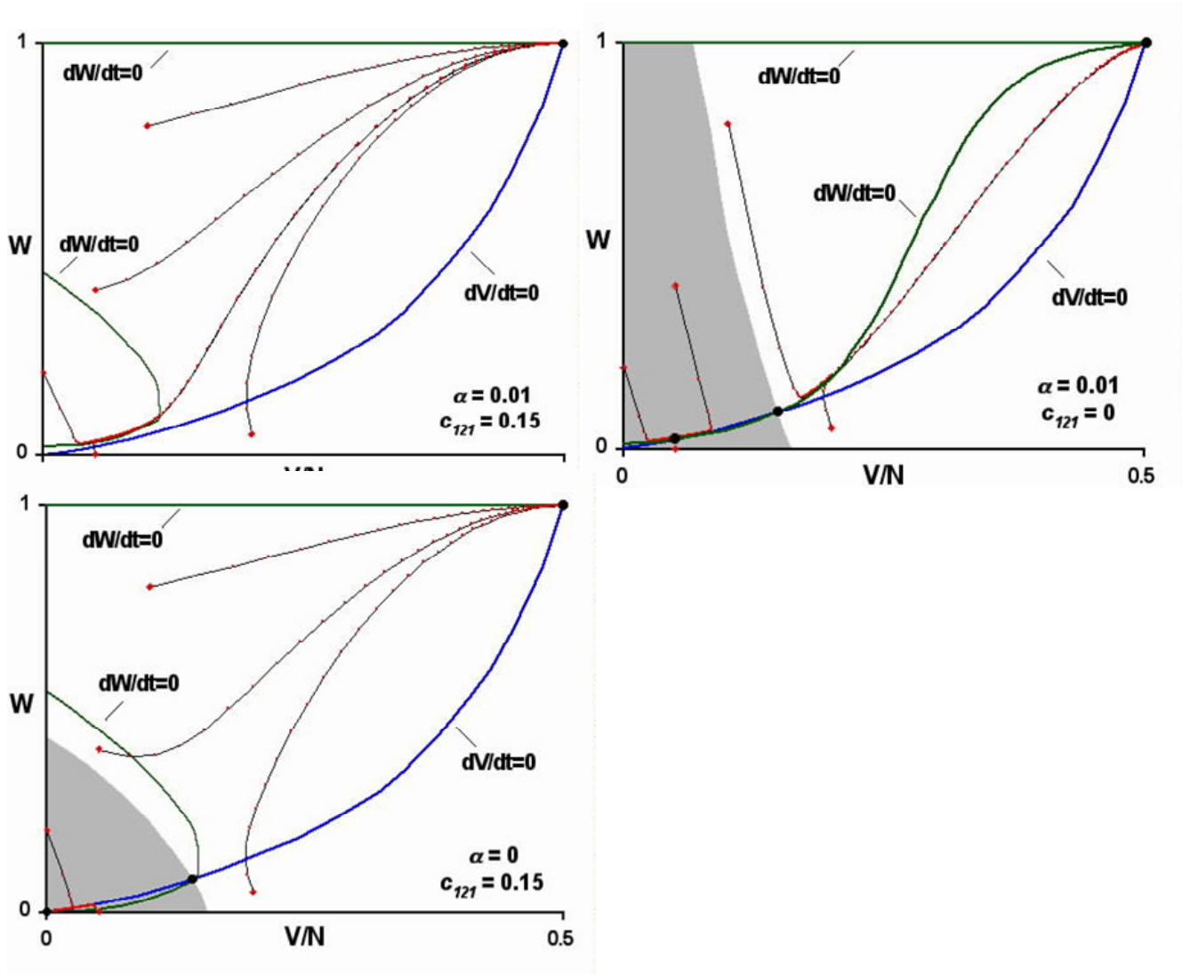
Figure 5 Phase space for two-dimensional system with endogenous willingness to consider and vehicle installed base. Fixed points exist at intersections of nullclines; dots show sample trajectories. Grey area shows basin of attraction for the low-diffusion equilibrium. Strength of marketing and nondriver word of mouth as shown. Other parameters as in Table 2.
