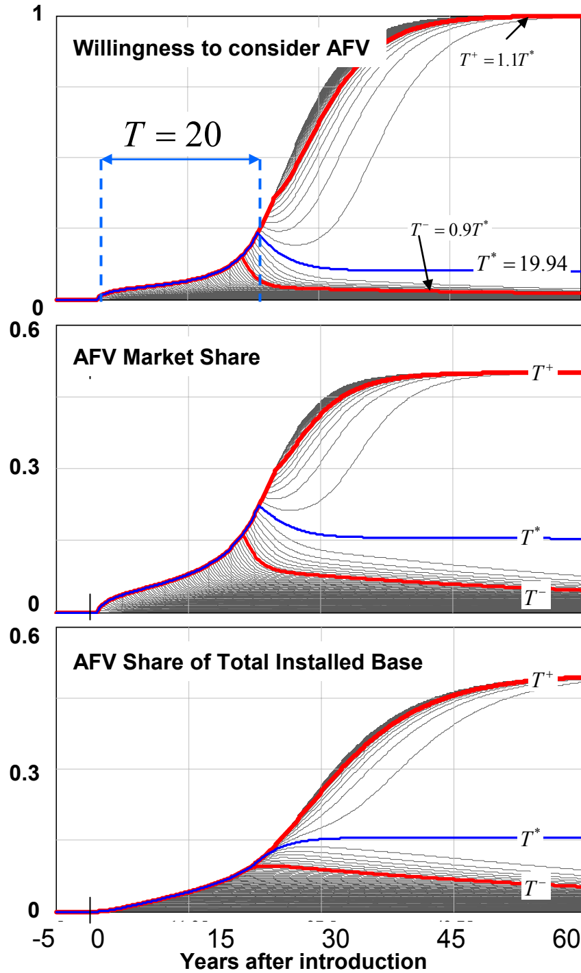
Figure 6 Willingness to consider alternative vehicle, sales- and installed base share with an aggressive marketing and promotion program. Duration of high marketing impact ( \alpha_2 = 0.025 ) varies between 0 and 50 years. Thick lines show the scenario for the critical marketing duration ( T^* = 19.94 years), and with a 10 percent increase and decrease of this.
